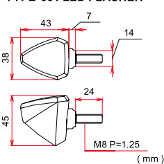
TYPE-601 LED FLASHER
