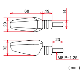
TYPE-602 LED FLASHER
