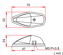
TYPE-586 LED FLASHER
